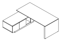
FS2001AR 200 - 90/180 - 74 FS2201AR 220 - 90/180 - 74
